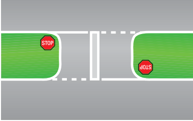
Stop hold lines
