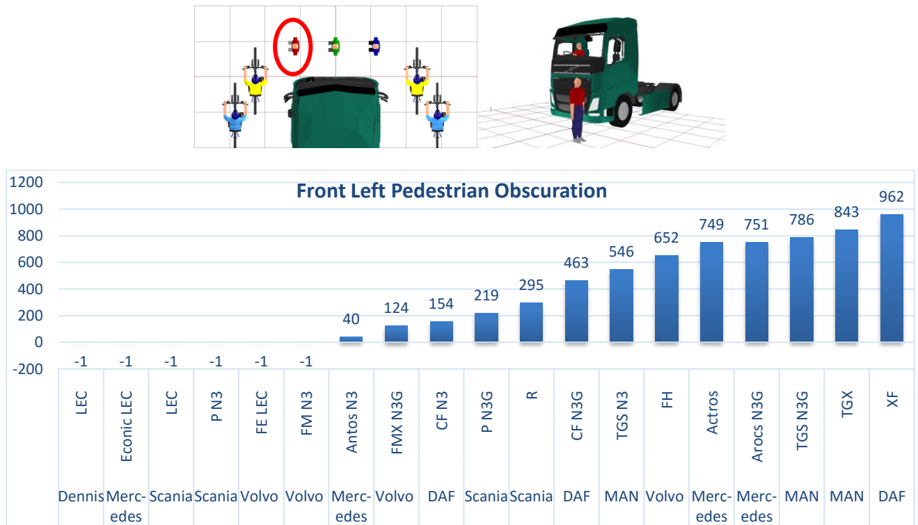
Figure 16. Graph showing the distance in millimetres from the front of the cab to the left pedestrian
