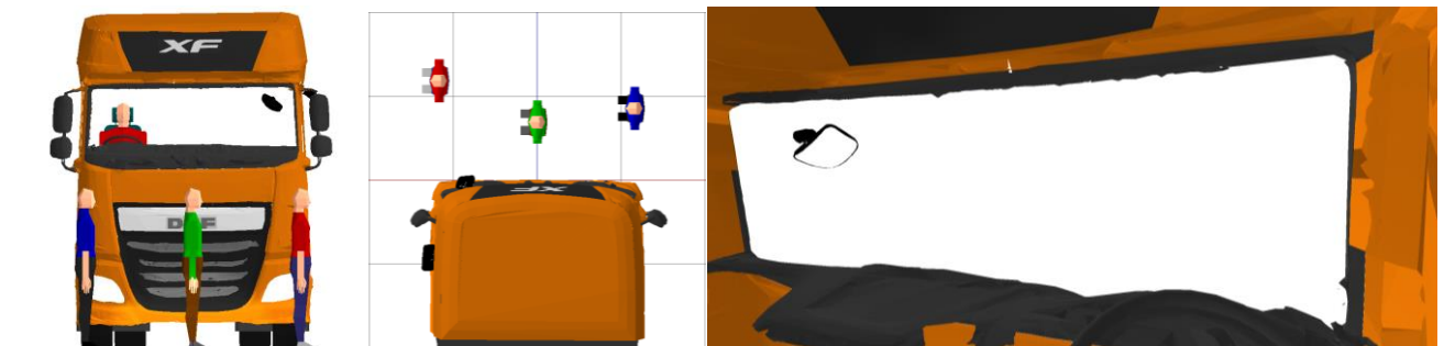
Figure 4. The direct field of view analysis to the front of the vehicle highlighting the position of the pedestrian models. The image to the left shows a front-on view of the vehicle. The image to the centre shows a top-down view. The image to the right shows the view from the driver's eyes through the windscreen.
