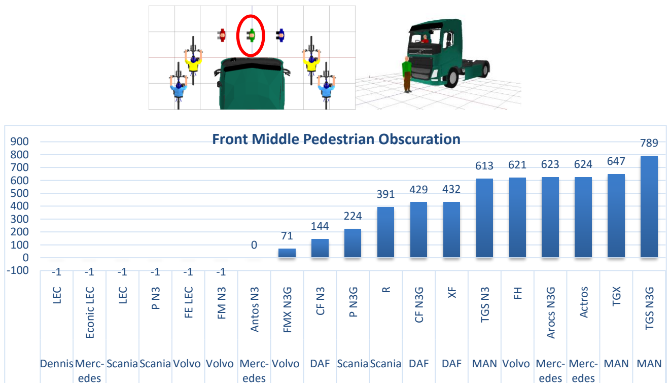
Figure 17. Graph showing the distance in millimetres from the front of the cab to the middle pedestrian
