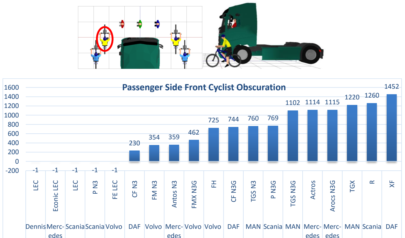
Figure 15. Graph showing the distance in millimetres from the side of the cab to the passenger side front cyclist
